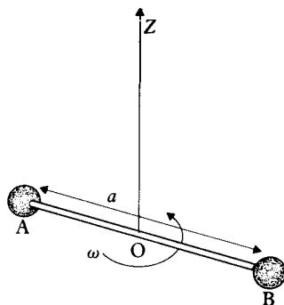
9.3 Rotation of a diatomic molecule composed of two nuclei A and B, each of the same mass M , a distance a apart. The rotation is of angular frequency \omega about an axis OZ through the centre of mass. The classical energy of rotation is E = \frac{1}{2}I\omega^2 , where the moment of inertia I is given by I = \frac{1}{2}Ma^2 .
